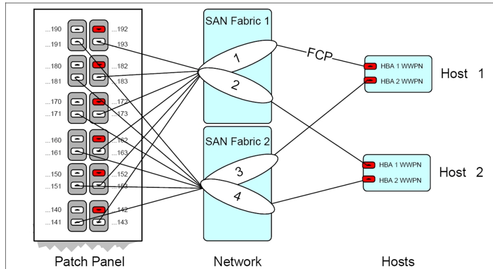
Figure 7. FC zoning: single initiator with multiple targets
