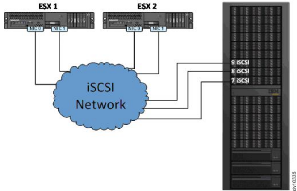
Figure 58. Connecting ESXi servers over iSCSI
