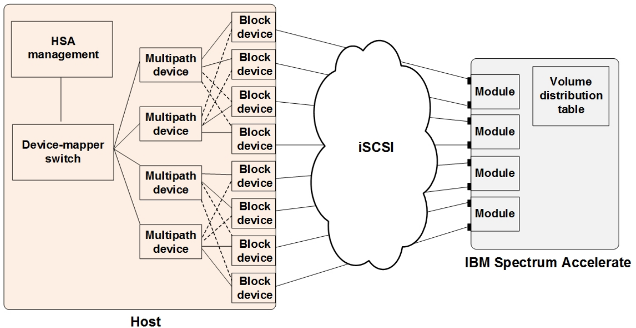
Figure 56. A host connected to IBM Spectrum Accelerate
