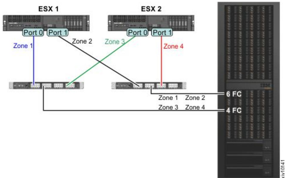
Figure 57. SAN Fibre Channel zoning layout
