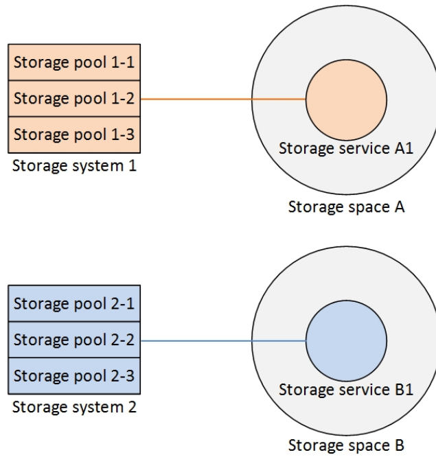
Figure 5. Single service per space and storage system
