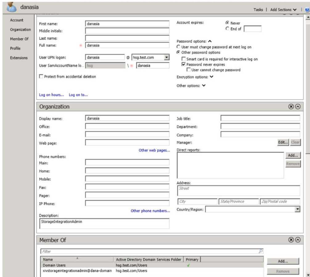
Figure 122. User configuration on Active Directory server
