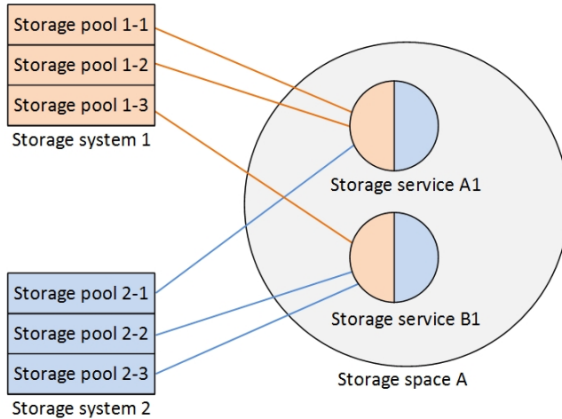
Figure 7. Multiple services per storage space and storage systems
