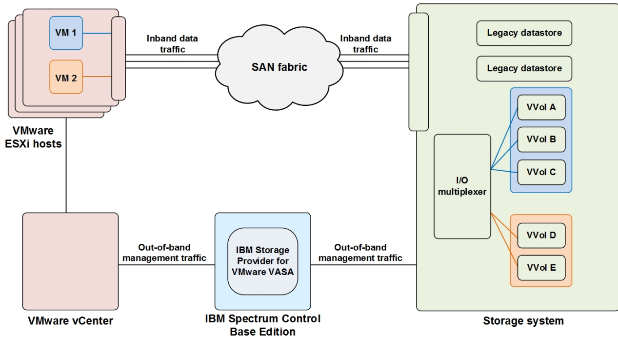
Figure 2. Using virtual volumes with IBM Spectrum Control Base Edition
