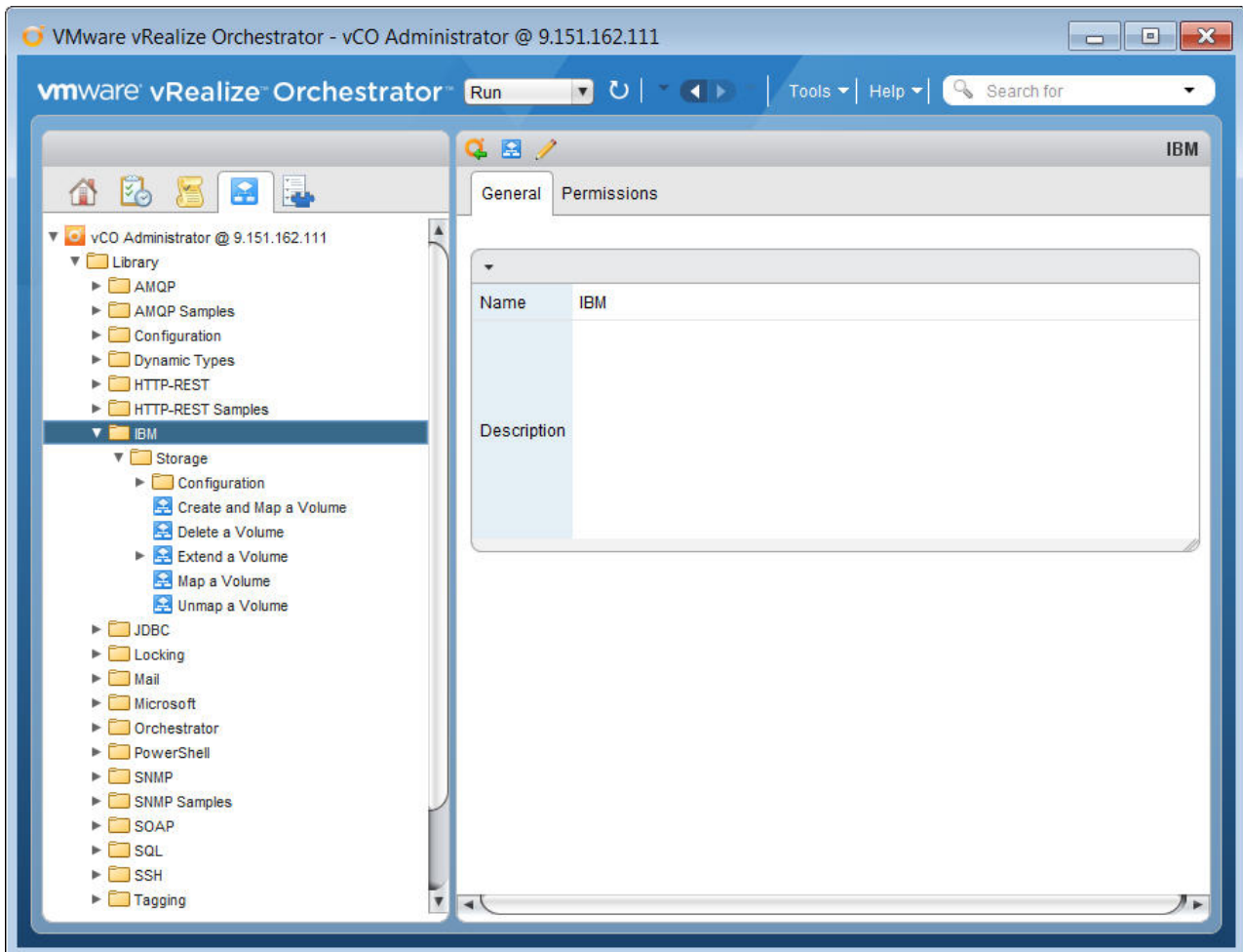
Figure 97. vRealize Orchestrator – available workflows – General tab
