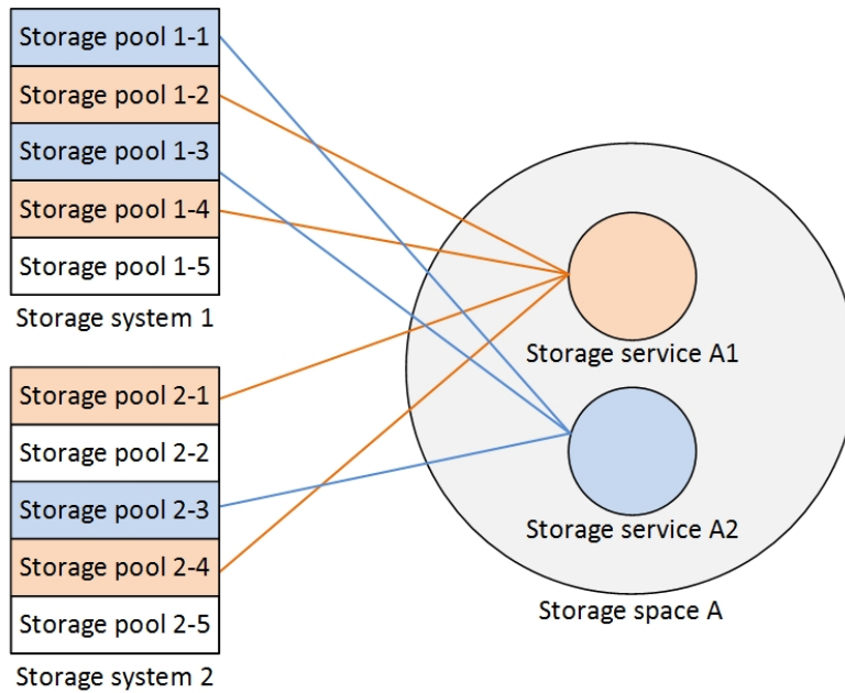
Figure 4. Storage elements without VVol utilization
