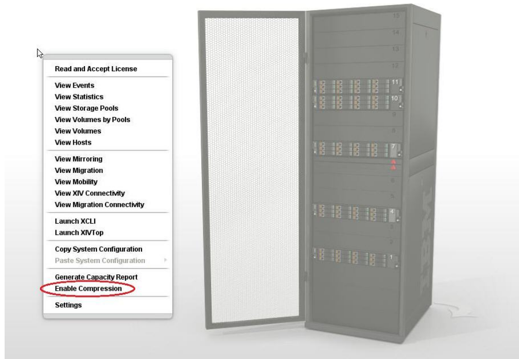
Figure 33. Enabling Compression
